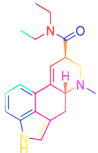
LSD Molecule
